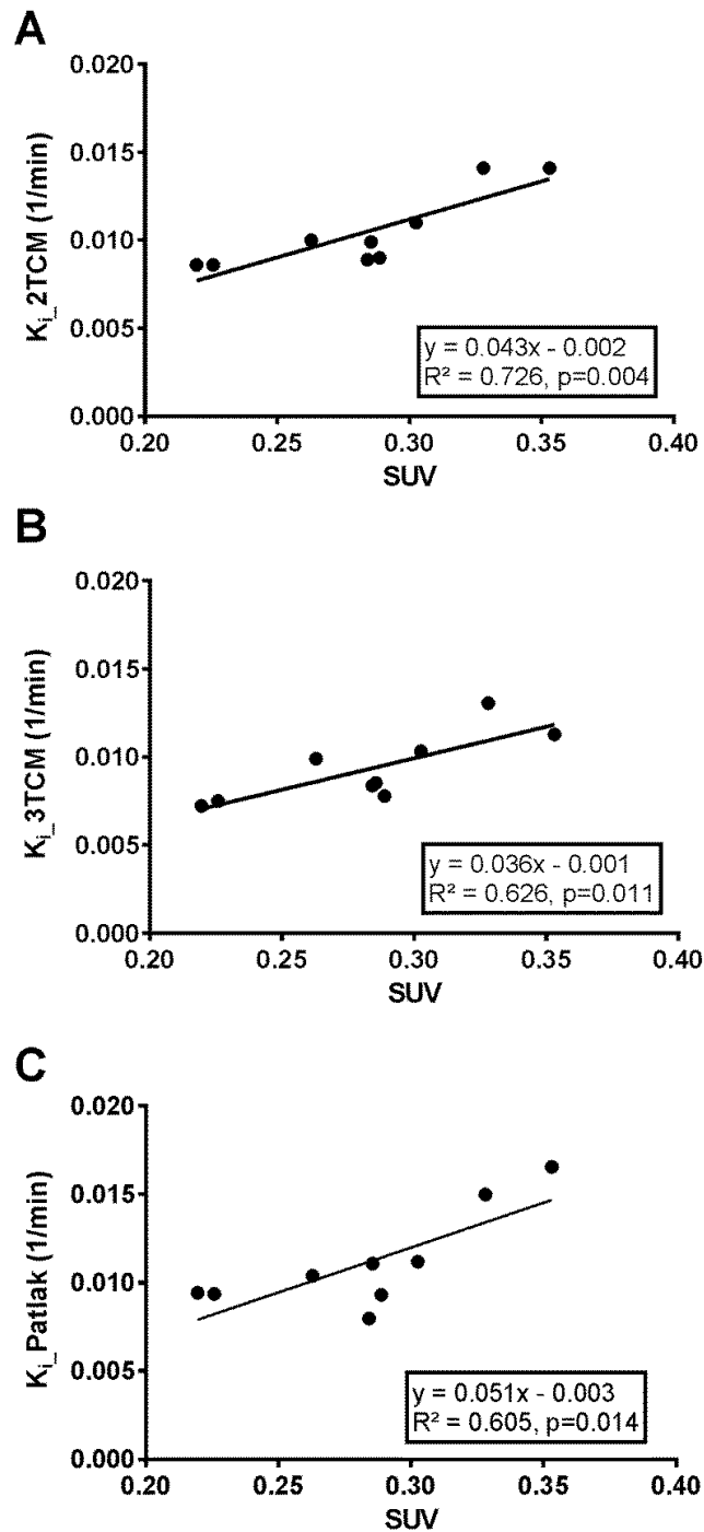
Supplemental figure 1. Correlation between SUV and K_i values from kinetic analysis using A) the 2TCM; B) the 3TCM or C) Patlak graphical analysis performed on the same tumors.
