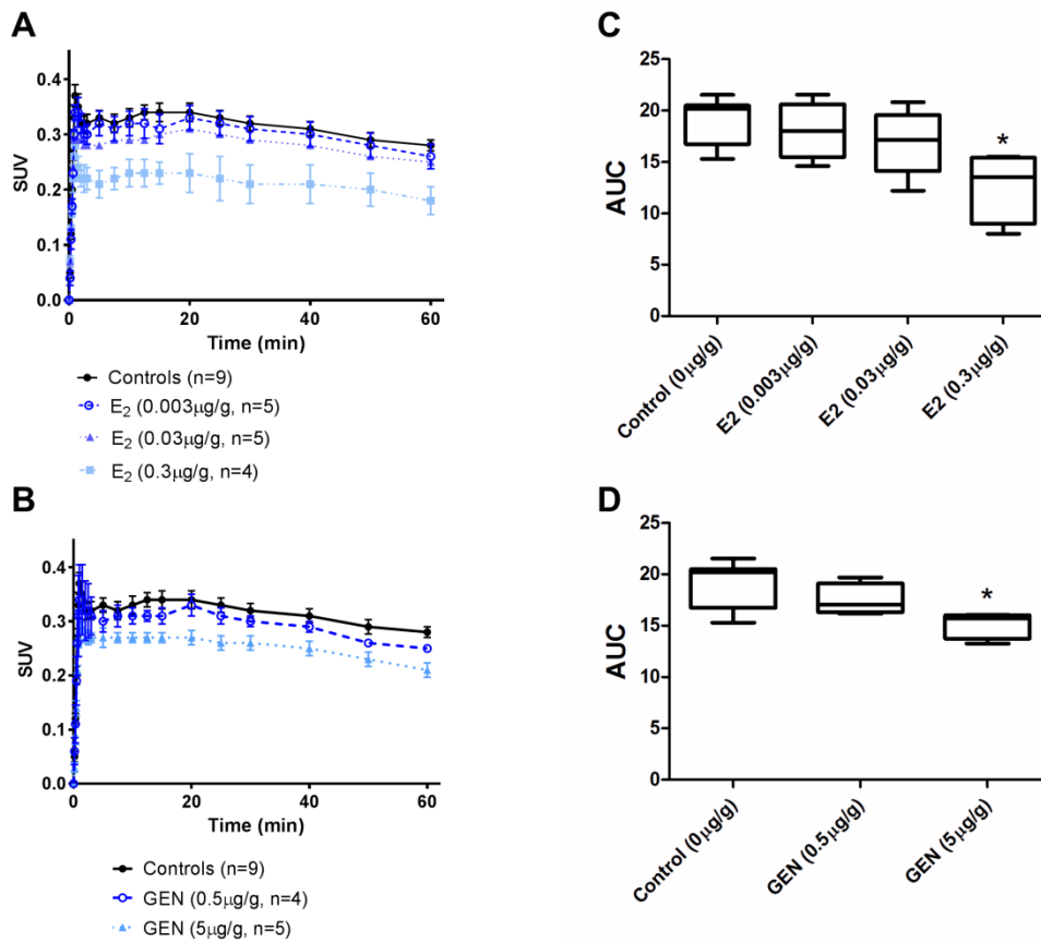
Supplemental figure 2. Kinetics of 18 F-FHNP in the SKOV3 xenografts. The effect of A) estradiol (E 2 ) and B) genistein (GEN) doses on tracer kinetics in the tumor over time. The effect of: C) estradiol and D) genistein on the area under the curve (AUC, min) for the different experimental groups. * p<0.05 when compared to the control group.
