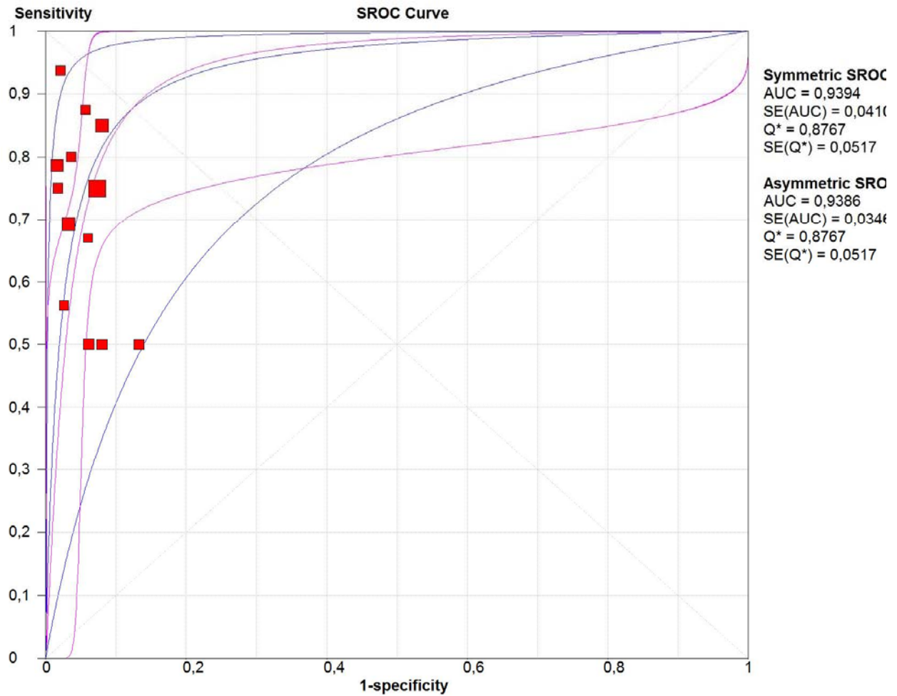
Supplemental Fig. 1: SROC's for LNM with confidence intervals: symmetric (in blue) and asymmetric (in pink).
