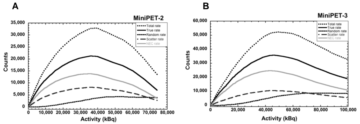
SUPPLEMENTAL FIGURE 1. Counting rate performance measured with the NEMA NU 4 rat phantom for the MiniPET-2 (A) and MiniPET-3 (B).
