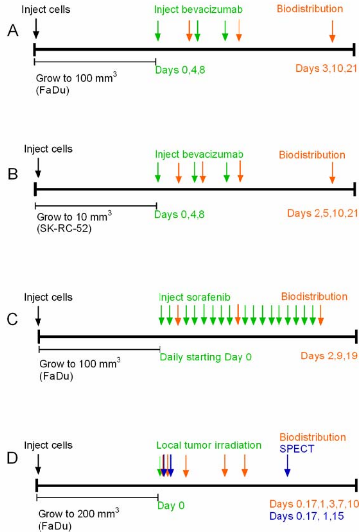
Supplemental Figure 1. Schedule of treatment regimes, biodistribution time points and SPECT imaging time points of mice bearing FaDu xenografts treated with bevacizumab (A), SK-RC-52 xenografts treated with bevacizumab (B), FaDu xenografts treated with sorafenib (C), or with local irradiation (D).
