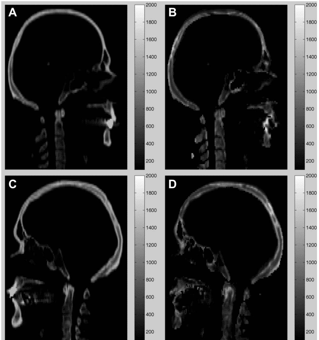
Supplemental Figure 1 – Sagittal views of CT for two patients (A,C) and corresponding MR-based density estimations (B,D). In this case, the available CT information was used to mask out all voxels below +100 HU. The UTE-derived R2 maps were then automatically rescaled to Hounsfield units.
