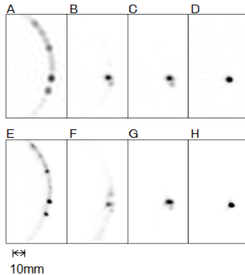
Supplemental Figure 3. Rotating rod source study showing the effect of time synchronization between motion tracking and scanner computers. The top row shows the images reconstructed with FBP for a rotating rod scan without motion correction (A), with MAF motion correction but without time synchronization (B), with MAF motion correction and with time synchronization (C), and a static rod scan (D). Each subframe has an intra-frame motion threshold (IFMT) of 2 mm and a minimum frame duration threshold (MFDT) of 3 sec, which keeps 32% of the scan data. The bottom row shows the images reconstructed with MOLAR for a rotating rod scan without motion correction (E), with EBE motion correction but without time synchronization (F), with EBE motion correction and with time synchronization (G), and a static rod scan (H). Time synchronization is necessary to enhance the accuracy of motion data, especially for the EBE motion correction method. B, C, D, F, G and H are displayed on a common scale, and A and E are displayed to a different scale to better visualize the effect of motion.
