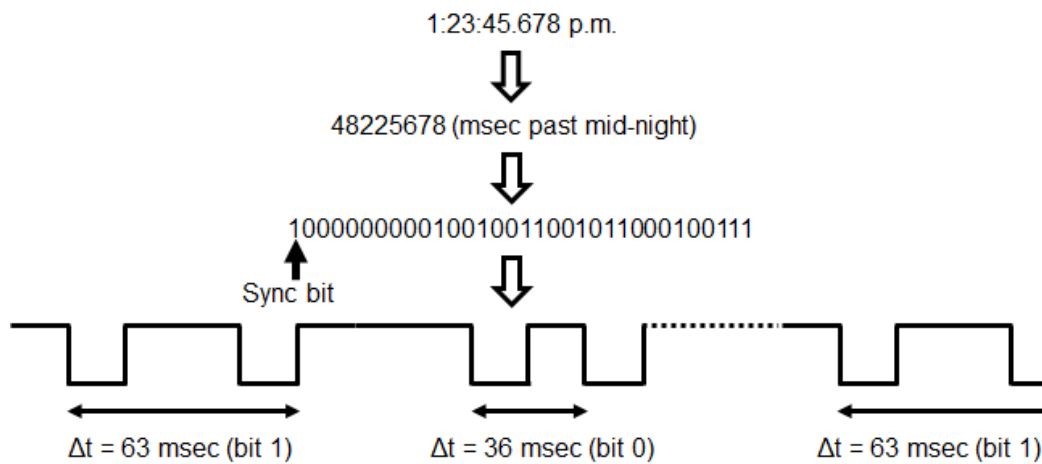
Supplemental Figure 1. Example of the time synchronization algorithm. The absolute time (in msec) past midnight is converted to an integer, which is represented in binary format. The bits are coded by two gating pulses separated by 36 or 63 msec for bit 0 or bit 1, respectively.
