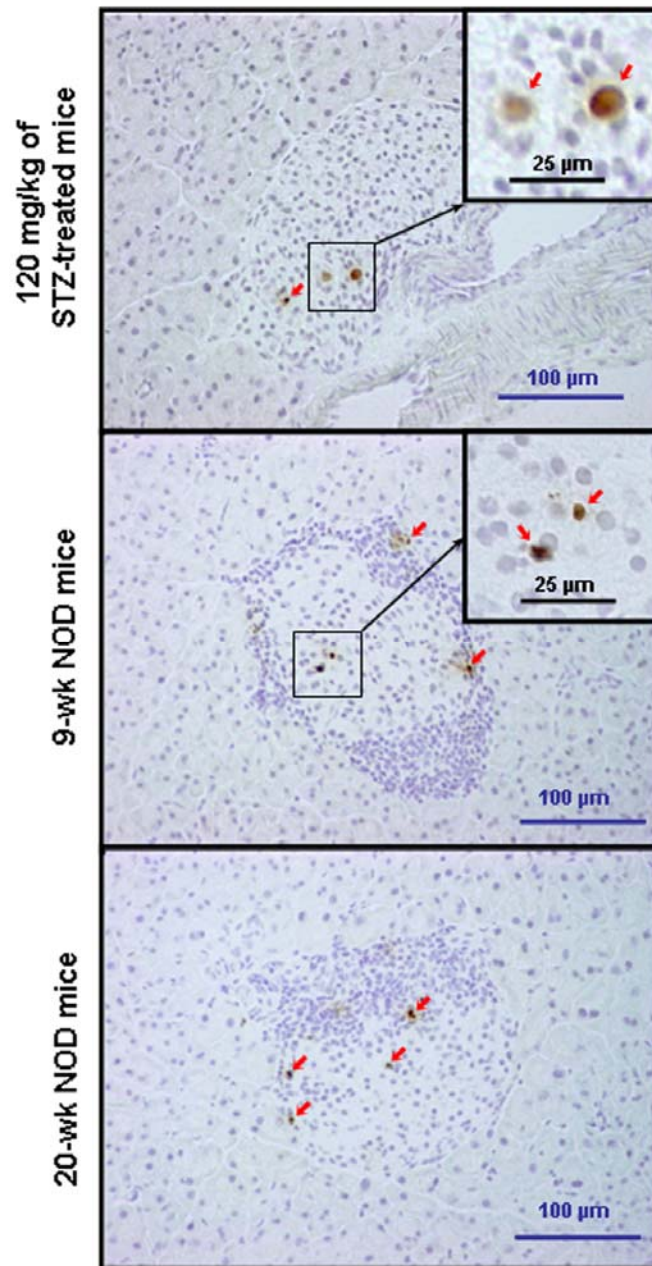
Supplemental Figure 1. TUNEL staining in the pancreas of STZ-treated mice and NOD mice injected with ^{99m}\text{Tc} -annexin A5. Arrows show TUNEL-positive cells. Boxes indicate the magnified areas shown in the insets. Blue scale bars: 100 \mu\text{m} , and black scale bars in inset: 25 \mu\text{m} .
