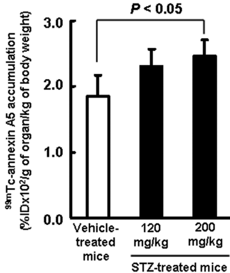
Supplemental Figure 2. Biodistribution of 99m Tc-annexin A5 in the pancreas of STZ-treated and vehicle-treated mice injected with 99m Tc-annexin A5. STZ-treated and vehicle-treated mice were injected with 99m Tc-annexin A5 (3.7 MBq/mouse). Six hours after the 99m Tc-annexin A5 injection, each pancreas was collected, weighed and measured for radioactivity using a gamma counter. Data represent mean \pm SD (n=4/group).
