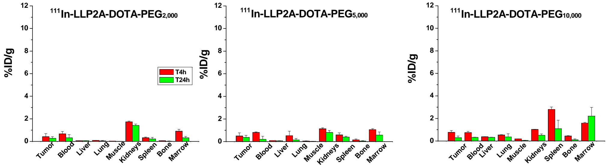
Biodistribution and tumor targeting of the 3 linear PEGylated monovalent ^{111}\text{In-LLP2A-DOTA} constructs.
