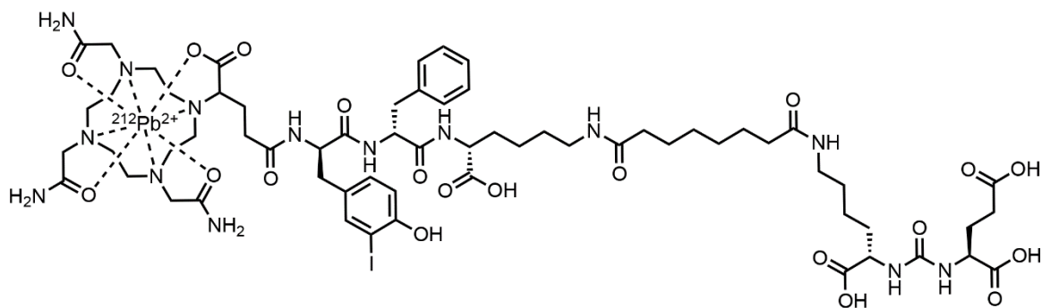
Structure of ^{212}\text{Pb} -ADVC001
