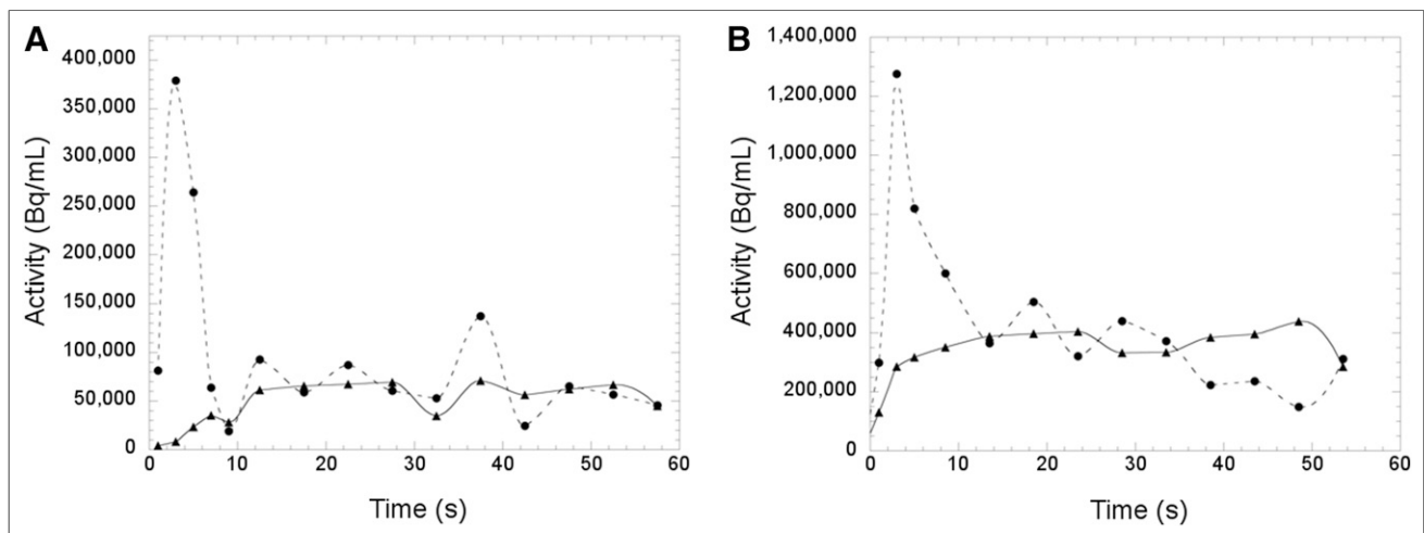
FIGURE 7. Time-activity curves were generated from both scanners by placing 1.5-mm-diameter spheric regions of interest within left ventricular blood pool and liver on serial short image frames during first 60 s of acquisition. Because injected activity was approximately 3 times higher on Inveon scanner than on Genisys4 scanner (2,072 and 629 kBq [56 and 17 \mu\text{Ci} ], respectively), vertical scales are different in A and B.
