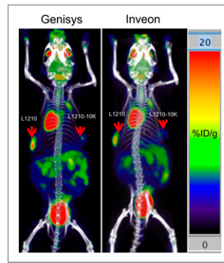
FIGURE 1. ^{18} F-FDG PET/CT maximum-intensity projections obtained with Genisys4 and Inveon PET scanners. L1210 and L1210-10K subcutaneous xenografts (red arrows) measured 8 and 6 mm in largest diameter; tumor uptake (%ID/g) was comparable (20.4 vs. 16.0 for L1210 and 7.5 vs. 6.7 for L1210-10K xenografts).
