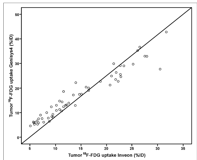
FIGURE 2. Correlation between ^{18} F-FDG tumor uptake measured with Inveon and Genisys4 scanners was highly significant ( y = 1.26x - 1.52 ; R^2 = 0.932 ; P < 0.001 ).
