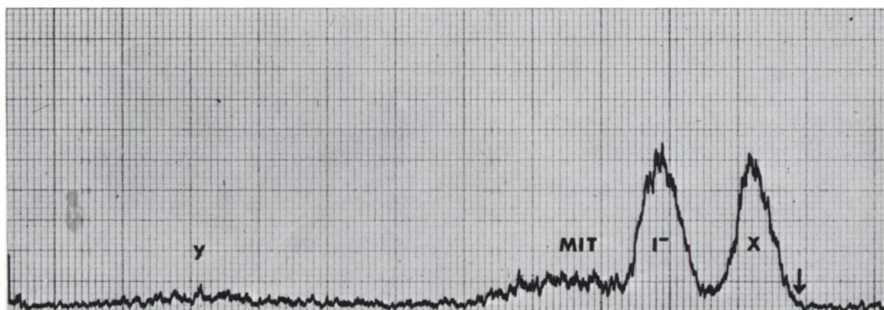
FIG. 2. Radiochromatogram of urine from euthyroid patient 0-6 hr after oral administration of MIT- 131 I. Butanol-acetic acid solvent system was used. Zones of labeled iodine correspond to x, iodide, MIT and y are shown. Arrow shows origin.
