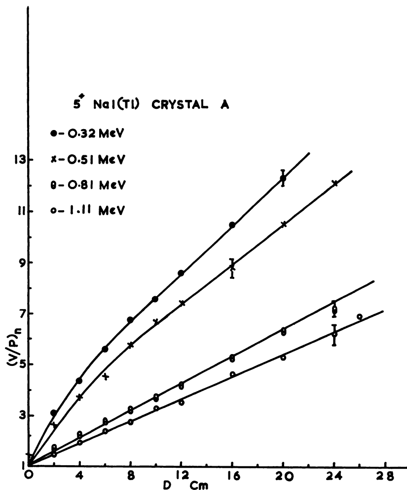
Fig. 2. Normalized valley-to-peak ratios for spectra obtained from a 5 inch NaI crystal for sources of different energy as the depth of water above the source is altered, the source—detector geometry being kept constant.
