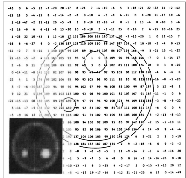
FIGURE 13. Computer simulation to evaluate Fourier transform reconstruction algorithm, 1-cm linear sampling resolution and 7.5 deg-angular sampling employed in PETT studies. Actual phantom is drawn on numerical printout with reconstructed image at bottom left-hand corner (image has right-to-left inversion from numerical printout). Actual values in 1-cm thick ring, 14-cm cylinder, 2-cm and 1-cm hot regions, and cold region were 300, 100, 500, 500, and 0, respectively.
