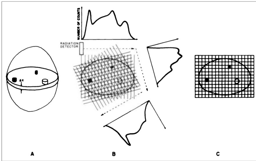
FIGURE 1. (A) Distribution of activity in cross-sectional slice of three-dimensional object. (B) Rectilinear scans performed at number of discrete angles around cross section of interest. Recorded data consists of activity profiles. (C) Reconstructed image formed by using data from activity profiles to mathematically solve for each element in grid or matrix representation.
