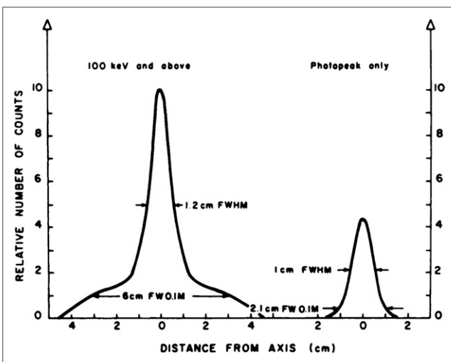
FIGURE 6. Line-spread function in water for ACD comparing difference between accepting energies of 100 keV and above to photopeak only. FWHM and FW 0.1 M are shown.
