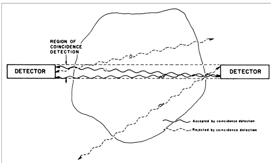
FIGURE 2. “Electronic” collimation of annihilation coincidence detection. Events are only recorded when two 511-keV photons emitted at 180 deg following positron annihilation are detected simultaneously.
