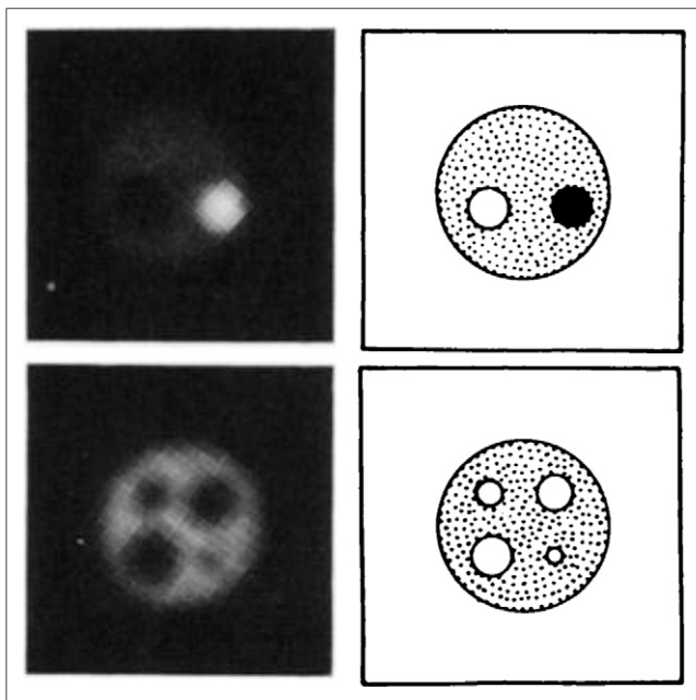
FIGURE 16. Top: test of quantitative reconstruction with PETT. Phantom consisted of 14-cm cylinder, 3-cm hot region, and 3-cm cold region with relative activities of 1, 4, and 0. Values in reconstructed images are 1 \pm 0.1 , 4 \pm 0.1 , and 0 \pm 0.1 . Image contained 340,000 counts. Bottom: test of cold spot reconstruction with PETT. Phantom consisted of 14-cm diam cylinder of activity with 3.5, 3, 2, and 1-cm voids (tubes filled with H_2O ). Image contained 300,000 total counts.
