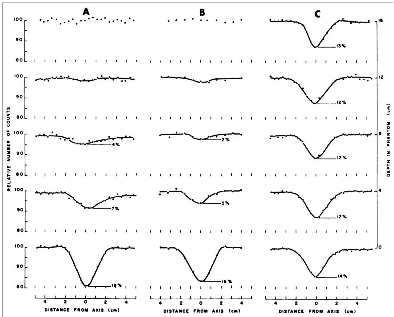
FIGURE 10. Comparison of cold spot scanning with 2.2-cm diam rod in water phantom containing either ^{99m}\text{Tc} or ^{64}\text{Cu} , for (A) scanner with absorption converging collimator (same counting system as used in Fig. 5, collimator-to-water bath distance 6 cm), (B) scintillation camera with 15,000-hole high-resolution collimator with water phantom placed against surface of collimator, and (C) annihilation coincidence system used for LSFs measurements in Fig. 4. Approximately same amount of activity and counting times were used in all cases.
