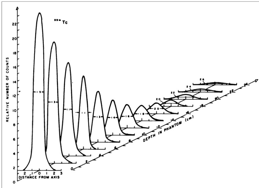
FIGURE 5. Line-spread function in water from SPC system. Detector system consisted of 2.5-cm diam X 5-cm thick NaI(Tl) and Ohio-Nuclear converging collimator No. 55035-L shielded down to 2.5-cm diam detector (interior 7 holes open). Collimator focal length was 12.7 cm; distance between collimator and water phantom was 4 cm.
