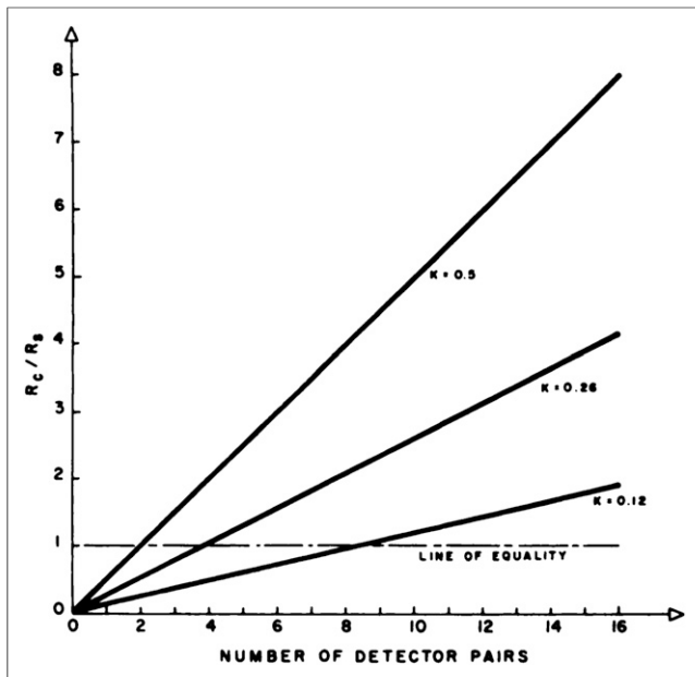
FIGURE 9. Plot of ratio of annihilation coincidence, R_c , to single photon, R_a , counting rates versus number of detector pairs, N . K is ratio of R_c to R_a for single pair of detectors. K = 0.12 and 0.26 are values for SPC system described in text to ACD system with photopeak only and 100 keV and above, respectively. K = 0.5 is given as a possible upper limit for optimal design for two systems. Line of identity indicates number of detector pairs required for systems to have equal efficiency.
