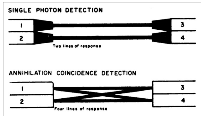
FIGURE 8. Illustration of N and N^2 dependence of efficiency for SPC and ACD, respectively, for multiple detector arrays. N is number of detector pairs.
