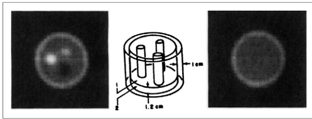
FIGURE 15. Evaluation of interference in reconstructed image taken with PETT from activity above level of interest. Center: schematic of split level phantom. Left: image taken at level 1 containing relative activities of 3, 1, 5, 3, and 0 in 1-cm ring, 14-cm cylinder, two 2-cm hot regions, and 3-cm cold region. Right: image taken from level 2 which contained only 1-cm ring and 14-cm cylinder and was 6 mm from center of level to above structure.
