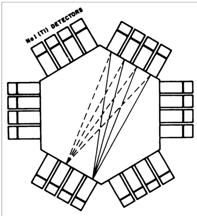
FIGURE 19. Schematic illustration of multiple coincidence logic possible with ACD of PETT.
