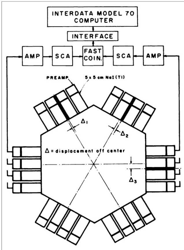
FIGURE 11. Schematic illustration of prototype PETT.
