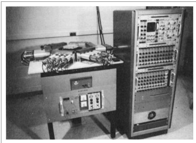
FIGURE 12. Photograph of prototype PETT. Object examined (phantom or animal) is placed on computer-controlled turntable at center of hexagon. Axis of rotation is perpendicular to plane of hexagon. Phantom is shown on turntable.
