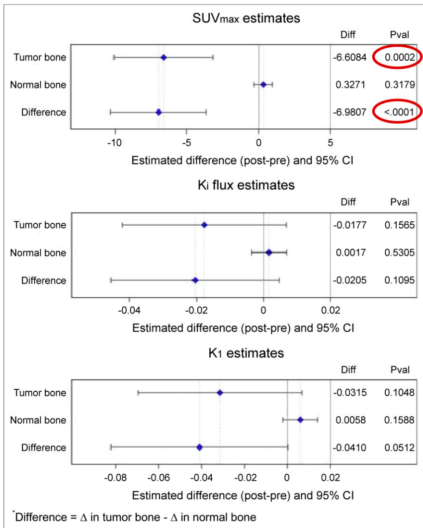
FIGURE 2. Change in regional fluoride incorporation occurred in response to dasatinib treatment in CRPC bone metastases when measured by SUV_{max} but not by K_{i,avg} . No significant changes were seen in response to dasatinib in normal bone. No significant changes in transport ( K_1 ) were observed after treatment with dasatinib. Diff = difference; Pval = P value.
