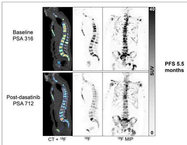
FIGURE 4. This patient had stable disease on bone and CT scan in response to dasatinib. Obvious heterogeneous changes in ^{18}\text{F} -fluoride PET response to dasatinib are detected, with decrease in ^{18}\text{F} -fluoride uptake in most bone metastases, yet L5 lesion appears to have increased uptake. MIP = maximum-intensity projection.
