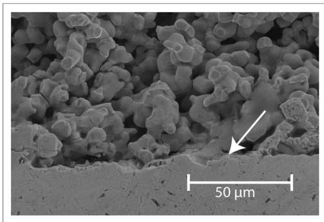
FIGURE 4. Scanning electron micrographs of target section. There is good bonding of molybdenum layer to tantalum target-backing plate (white arrow). Deposited material is porous as noted by voids in deposited target material.
