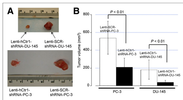
FIGURE 7. Suppression of tumor growth by knockdown of hCtr1 in human prostate cancer xenografts in mice. (A) Tumors with knockdown of hCtr1 (Lenti-hCtr1-shRNA-PC-3 tumor and Lenti-hCtr1-shRNA-DU-145 tumor) were smaller than those without knockdown of hCtr1 (Lenti-SCR-shRNA-PC-3 tumor and Lenti-SCR-shRNA-DU-145 tumor), at 4 wks after implantation of PC-3 cells and 7 wks after implantation of DU-145 cells, respectively. (B) Volumes of tumors with knockdown of hCtr1 (Lenti-hCtr1-shRNA-PC-3 and Lenti-hCtr1-shRNA-DU-145) were significantly smaller than those without knockdown of hCtr1 (Lenti-SCR-shRNA-PC-3 and Lenti-SCR-shRNA-DU-145), based on calculation from tumor size measured ex vivo with caliper. Error bar, SD.
