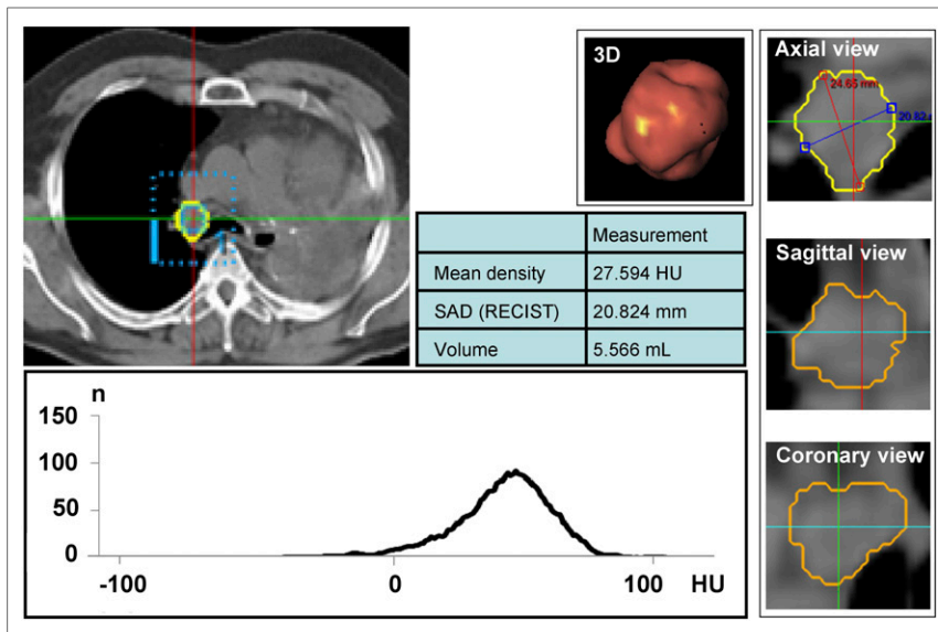
FIGURE 2. 3D evaluation of mediastinal lymph node metastasis. For computing histograms, semiautomatic method was used (Fraunhofer MEVIS). Within estimated region of interest, thresholds were generated automatically by segmentation software. For validation, semiautomated results were verified using implemented 3D viewer for multiplanar reconstruction (images on right). Spatial parameters were extracted, and histogram of all voxels in segmented lymph node was generated (graph at lower left). RECIST = Response Evaluation Criteria in Solid Tumors.
