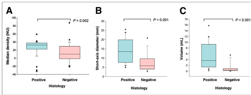
FIGURE 4. Box-and-whisker-plot analysis. (A) CT density of lymph node on nonenhanced CT. On the basis of CT density, affected and nonaffected lymph nodes presented significantly different density values on CT imaging. Histologically positive (affected) lymph nodes had median CT density of 33.2 HU, whereas histologically negative (nonaffected) lymph nodes had median CT density of 10.1 HU ( P = 0.002 ). (B) SAD of lymph node. On nonenhanced CT scans, positive lymph nodes had median SAD of 13.5 mm. SAD was significantly smaller in negative lymph nodes, which had median SAD of 5.8 mm ( P < 0.001 ). (C) Volume of lymph node. Affected lymph nodes (positive) had higher volume than nonaffected lymph nodes (negative) ( P < 0.001 ).
