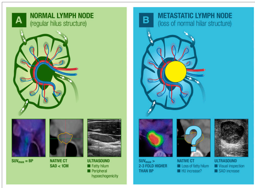
FIGURE 1. Normal and metastatic lymph nodes with specific characteristics on ultrasound, PET, and CT. (A) Schematic illustration of normal lymph node with corresponding findings on PET/CT ( ^{18}\text{F} -FDG-negative), ultrasound (slim shape with peripheral halo sign), and exemplary nonenhanced CT. (B) Schematic picture of lymph nodes with metastatic infiltration, showing positive ^{18}\text{F} -FDG uptake on PET/CT. Exemplary round metastatic lymph node on ultrasound with loss of hilar architecture and rare calcifications. BP = blood pool.
