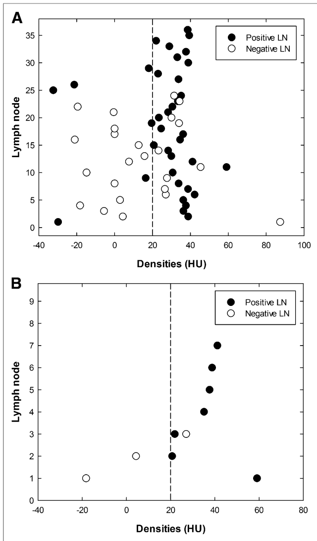
FIGURE 5. Mean histogram and density spread. (A) Density spread of affected lymph nodes (positive) vs. nonaffected lymph nodes (negative). Seventy-seven percent of lymph nodes with density higher than 20 HU were malignant; 82% of lymph nodes with density below 20 HU were benign. (B) Density spread in subgroup of 18 F-FDG-equivocal lymph nodes: 100% of lymph nodes below 20 HU cutoff were benign (negative); 88% of lymph nodes with density above 20 HU were malignant (positive). LN = lymph node
