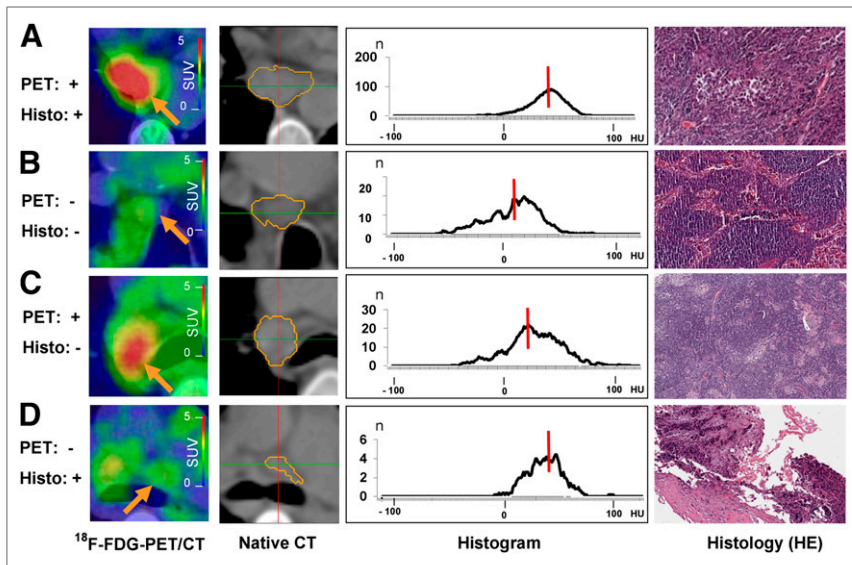
FIGURE 3. Comparison of ^{18}\text{F} -FDG PET/CT, nonenhanced CT, 3D CT histogram analysis with median density values (red lines), and histologic cross sections (hematoxylin and eosin [HE], \times 40 ). (A) Patient with adenocarcinoma. PET-positive malignant lymph node is at position 7 (SAD, 19 mm; volume, 1.6 \text{cm}^3 ). Median density of 31 HU in related CT histogram is beyond possible cutoff of 20 HU. Histologic cross section shows lymph node tissue with sparse infiltrates of atypical epithelial cells. (B) Patient with adenocarcinoma. PET-negative benign lymph node is at position 4R (SAD, 11 mm; volume, 0.9 \text{cm}^3 ). Corresponding CT histogram has median density of 12 HU. Histologic cross section shows prominent sinus histiocytosis and no evidence of malignancy. (C) Patient with adenocarcinoma. PET-positive benign lymph node is at position 10R (SAD, 20 mm; volume, 1.5 mL). Corresponding CT histogram has median density of 21 HU. Histologic cross section shows regular lymph node tissue, few sarcoidlike lesions, and slight lymphofollicular hyperplasia. (D) Patient with large cell neuroendocrine tumor. PET-negative lymph node is at position 4L (SAD, 7 mm; volume, 1 mL). Corresponding CT histogram has median density of 28 HU. Histologic cross section shows sparse lymph node tissue and desmoplastic stroma with focal non-small cell lung cancer (upper left corner).
