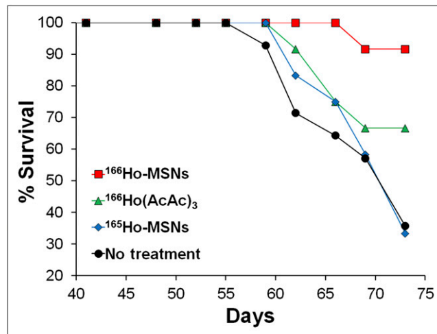
FIGURE 4. Survival of ovarian tumor-bearing mice after intraperitoneal administration of nonirradiated ^{165}\text{Ho-MSNs} , ^{166}\text{Ho-MSNs} , ^{166}\text{Ho(AcAc)}_3 , or no treatment. All administrations were 20 d after intraperitoneal implantation of 15 \times 10^6 SKOV-3 human ovarian tumor cells.
