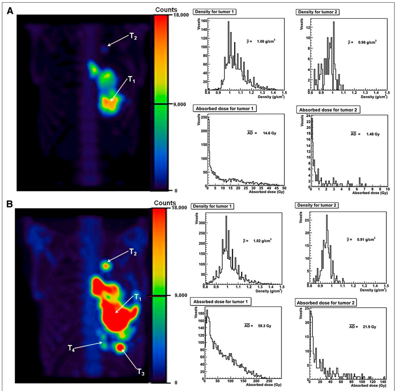
FIGURE 1. Example of 3D-RD analysis. Four hours after low-dose ^{153}\text{Sm} -EDTMP SPECT for patient 2, 2 tumors were identified ( T_1 and T_2 ) for dosimetry analysis (A). Density and dose–volume histograms for tumors are also shown. Four hours after high-dose ^{153}\text{Sm} -EDTMP SPECT for same patient, 2 new tumors ( T_3 and T_4 ) were identified in addition to 2 tumors identified at low-dose therapy (B). Tumor density and dose–volume histograms for 2 old tumors ( T_1 and T_2 ) seen at low-dose therapy are shown for comparison. SPECT images are shown, with same maximum intensity for comparison. AD = absorbed dose.
