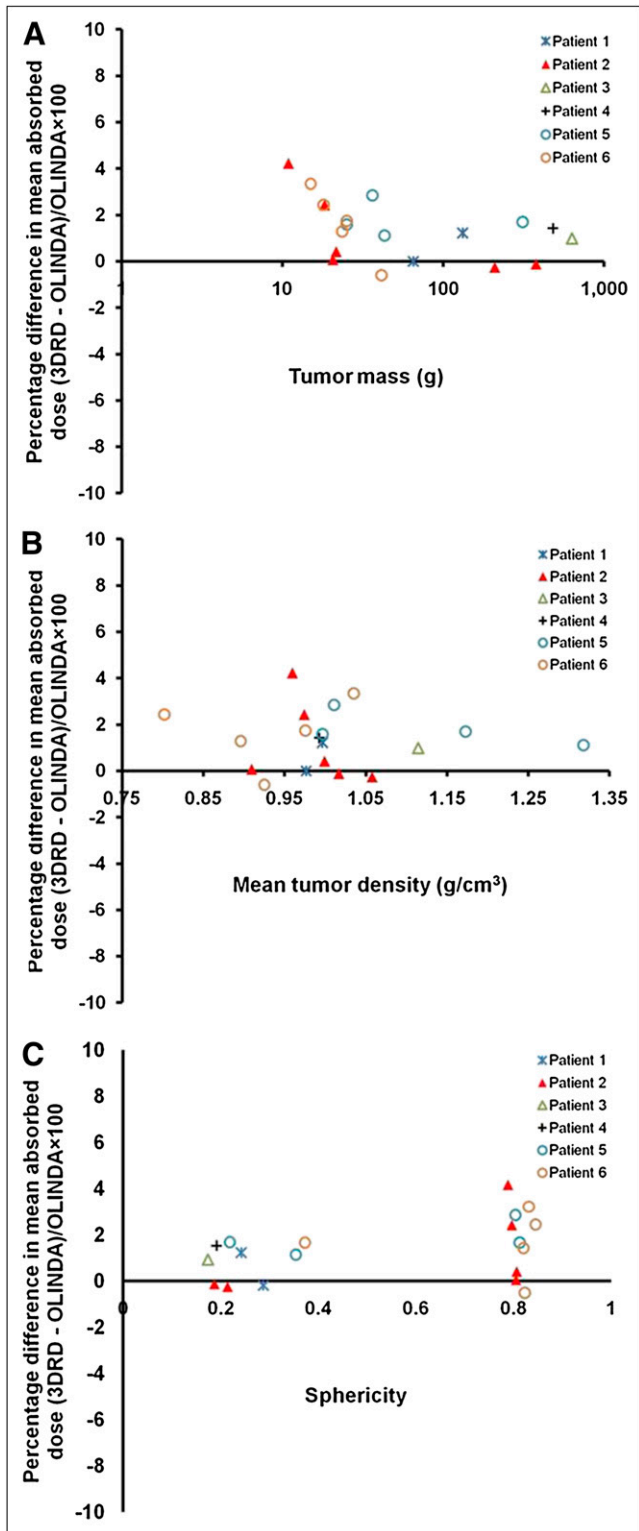
FIGURE 4. Comparison of percentage difference in mean absorbed dose estimates between 3D-RD and OLINDA/EXM unit-density sphere model as function of individual patient tumor mass (A), density (B), and sphericity (C). Tumor mass is in logarithmic scale in A.
