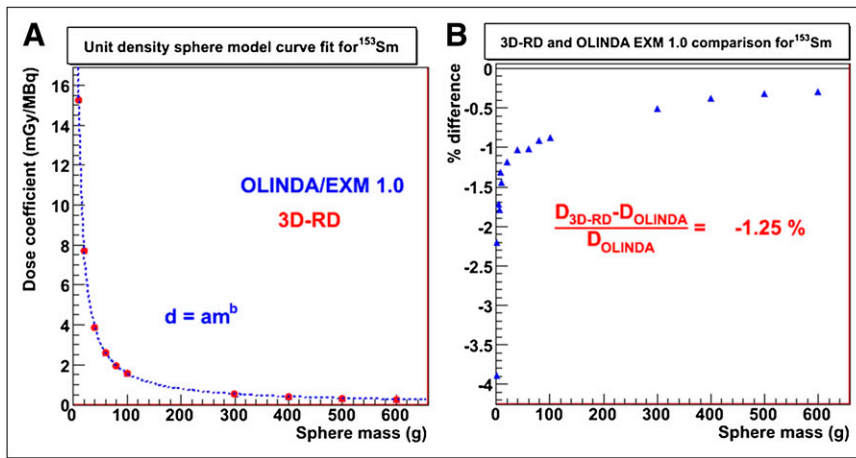
FIGURE 3. Mean absorbed dose calculation based on unit-density sphere model. (A) Power-law fit (dotted line) to OLINDA/EXM dose coefficients against ^{153}\text{Sm} -filled homogeneous unit-density spheres of various masses (1–600 g) is demonstrated. 3D-RD-generated dose coefficients are shown as solid point for each sphere on curve fit for comparison. (B) Percentage difference between 3D-RD and OLINDA/EXM for each sphere is given.
