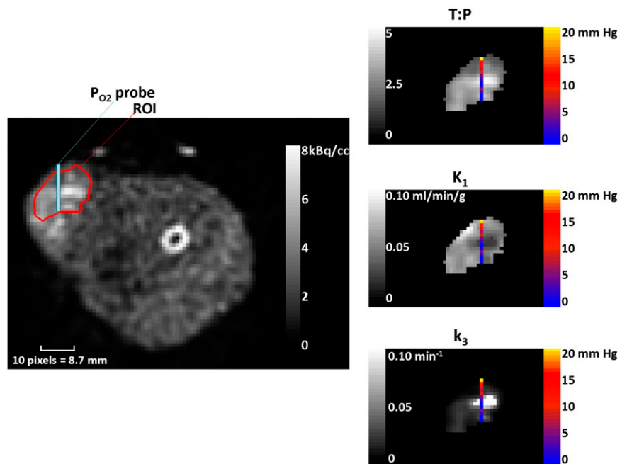
FIGURE 3. On left is image averaged over last 40 min, with ROI used to segment data for kinetic analysis overlaid in red and \text{Po}_2 probe trajectory overlaid in blue. Images on right are voxelwise kinetic maps for same slice and ROI shown on left. Overlaid onto each of these maps are corresponding \text{Po}_2 concentration measurements made at each of those corresponding voxel locations.
