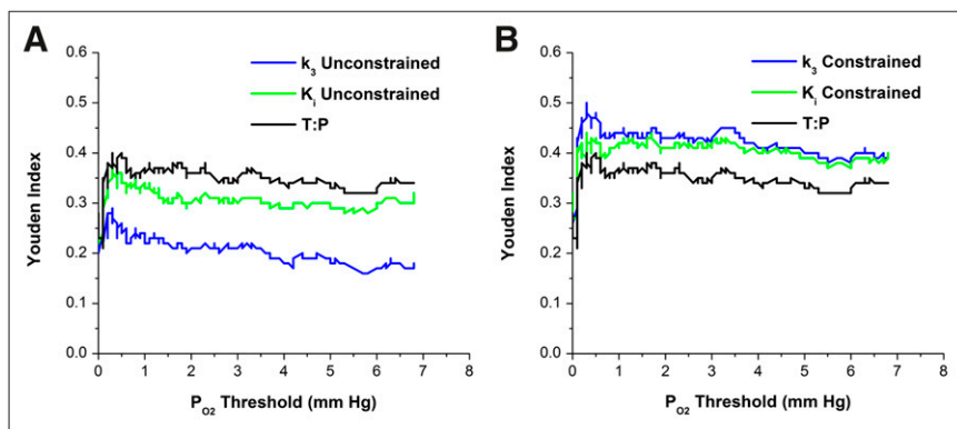
FIGURE 5. Plots of Youden index vs. \text{Po}_2 threshold: unconstrained model (A) and constrained model (B).
