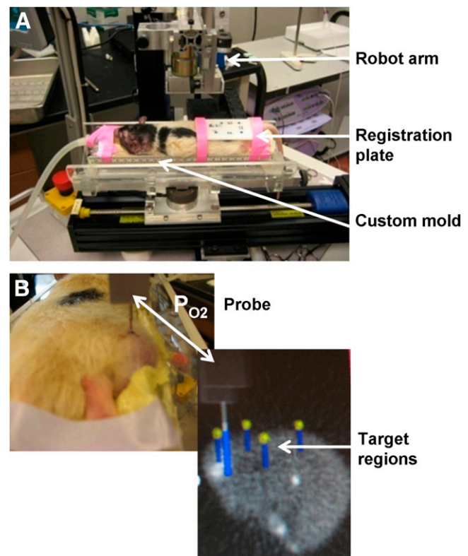
FIGURE 1. (A) Anesthetized rat immobilized in custom-fabricated foam mold, positioned on robot platform. Registration plate is centered over rat tumor. (B) Top image is rat tumor with OxyLite probe sampling \text{Po}_2 along predefined track. Bottom image is target region for sampling \text{Po}_2 as defined on 5-min static PET image.
