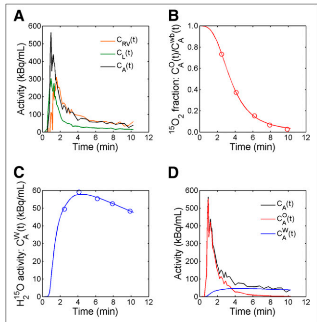
FIGURE 1. Ascending aorta, right ventricle, and lung time–activity curves (A), ratio of ^{15}\text{O}_2 to whole-blood concentrations (B), compartment model fit of ^{15}\text{O} -water radioactivity concentration in blood (C), and resulting ^{15}\text{O}_2 and ^{15}\text{O} -water input functions (D) for typical patient during ^{15}\text{O}_2 inhalation.
