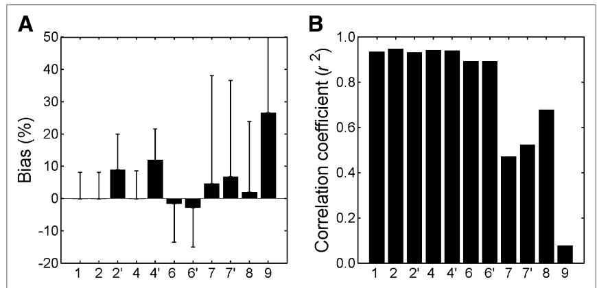
FIGURE 2. Simulation study: mean bias ( \pm SD) of fitted OEF relative to true (simulated) OEF (A) and correlation coefficient ( r^2 ; B) between fitted and true values for all models.
