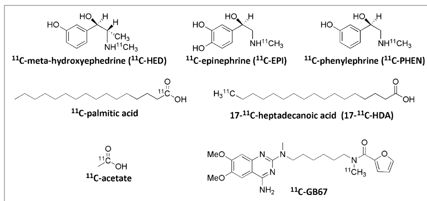
FIGURE 7. Selected ^{11}\text{C} PET radiotracers for cardiac imaging.
