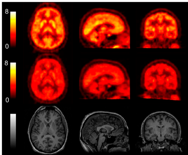
FIGURE 1. Representative PET images after ^{11}\text{C} -GSK189254 administration to a healthy human subject before (top) and 4 h after (middle) a 50- \mu\text{g} oral dose of GSK189254. Mean standardized uptake value images over 0–90 min are shown with structural MR image for same subject (bottom).
