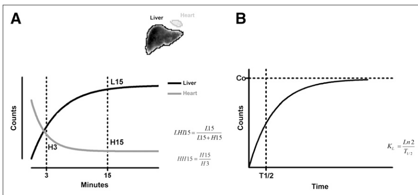
FIGURE 1. Planar dynamic 99m Tc-GSA scintigraphy. (A) LHL15 and HH15 are calculated from 99m Tc-GSA time-activity curves from heart (gray) and liver (black). (B) Blood clearance constant ( K_L ) is calculated from liver uptake curve using clearance half-time ( T_{1/2} ).
