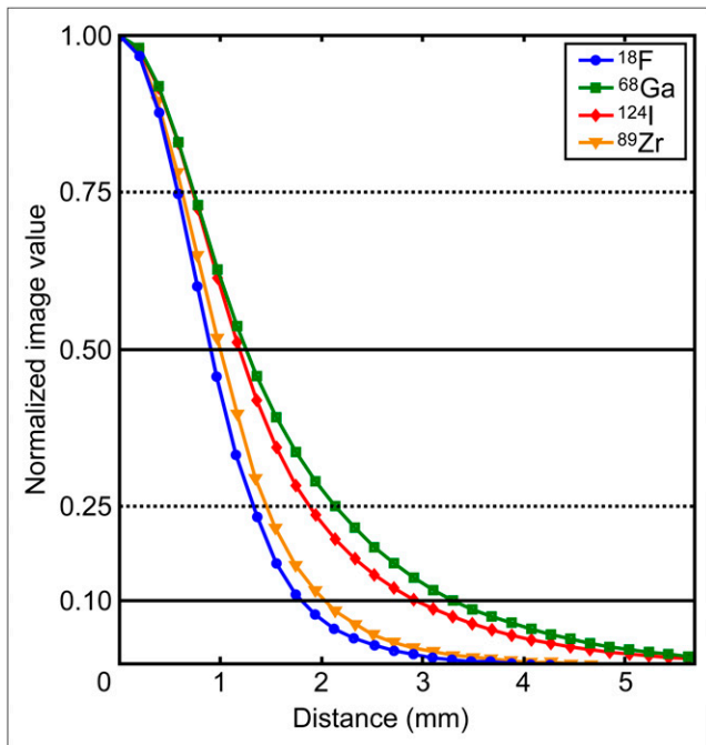
FIGURE 2. Measured line profiles through glass capillaries filled with positron-emitting aqueous solutions, surrounded by water. Profiles were obtained from 512 \times 512 FBP reconstruction by aligning and summing image slices containing capillary and averaging profiles in tangential and radial directions through center. Profiles are shown in 1 direction only. Values were not corrected for source dimensions.
