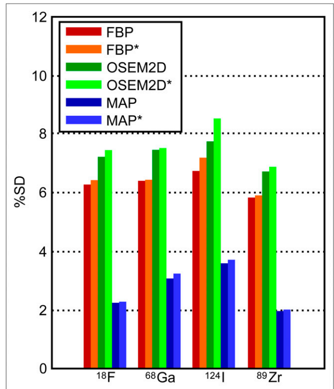
FIGURE 3. %SD in uniform phantom region. *Reconstruction performed with scatter correction.
