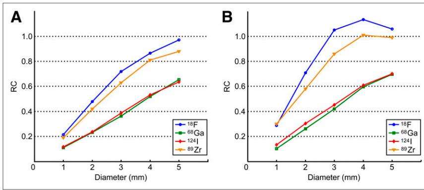
FIGURE 4. RCs of different rods for various radionuclides, reconstructed with FBP (A) and MAP (B). OSEM2D results were similar to those of FBP.
