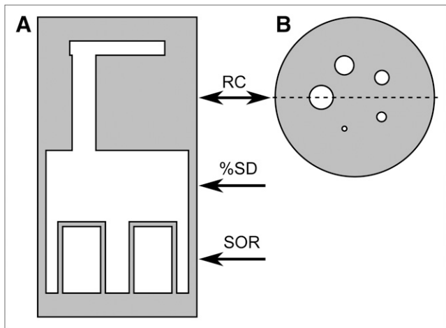
FIGURE 1. Cross-sectional diagram of NEMA NU 4 image-quality phantom. Gray represents solid polymethylmethacrylate, and white represents hollow, fillable compartments. Views are coronal (A) and transverse through rod (B).
