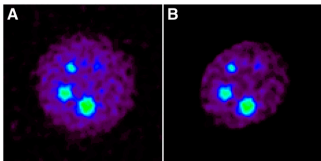
FIGURE 6. Transverse cross-section through rod area of phantom filled with ^{124}\text{I} solution. Images without (A) and with (B) scatter correction are shown. Scatter-corrected image clearly displays ellipsoid deformation.
