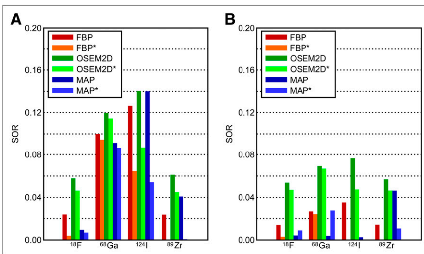
FIGURE 5. SORs in water (A) and air (B) compartments for various radionuclides, reconstructed with 3 different algorithms. Some SOR values are (close to) zero, and not visible in graph. *Reconstruction performed with scatter correction.
