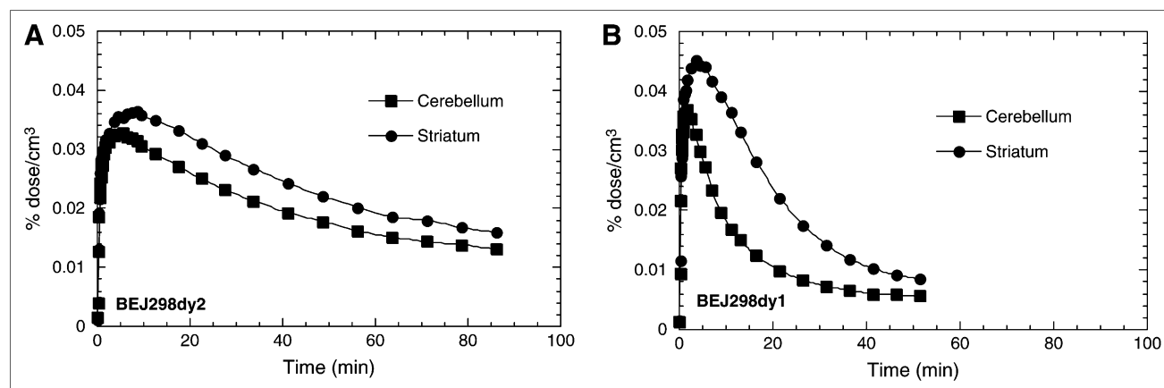
FIGURE 4. Time-activity curves for ^{11}\text{C} - d -methamphetamine (A) and ^{11}\text{C} -(-)-cocaine (B) in cerebellum and striatum in same baboon (BEJ298dy1 and BEJ298dy2 refer to study number). Clearance of ^{11}\text{C} - d -methamphetamine is lower and slower than that of ^{11}\text{C} -(-)-cocaine.
