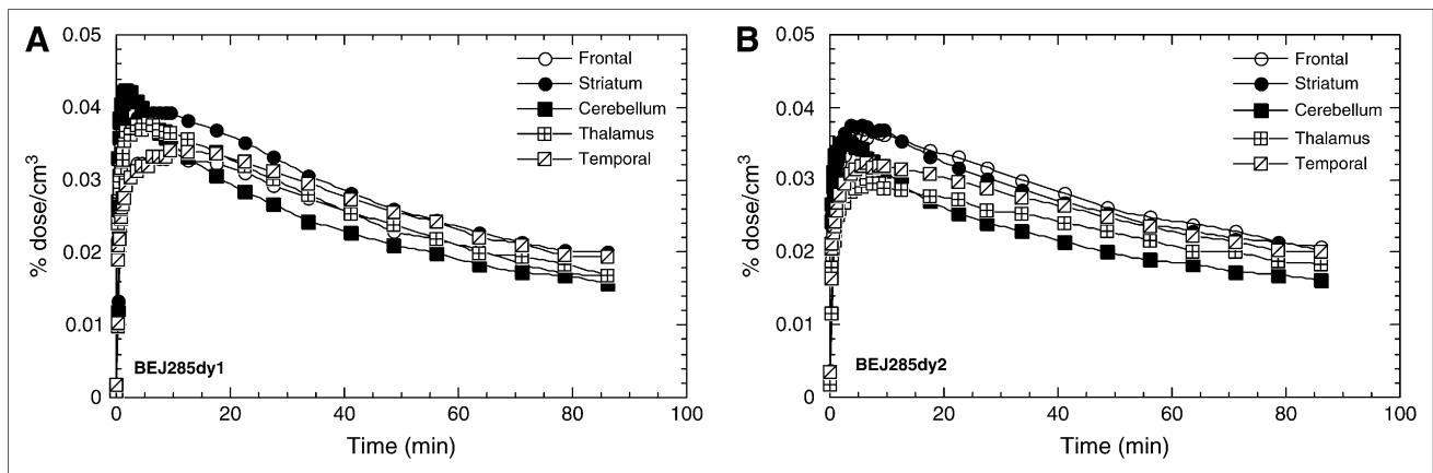
FIGURE 2. Time-activity curves for cortical and subcortical brain regions for ^{11}\text{C} - d -methamphetamine (A) and ^{11}\text{C} - l -methamphetamine (B) in same baboon (BEJ285dy1 and BEJ285dy2 refer to study number). Brain kinetics are similar for different brain regions.
