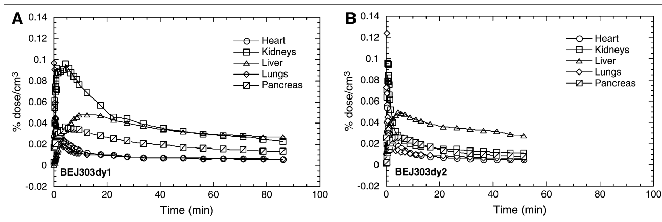
FIGURE 5. Comparison of distribution and clearance of 11 C- d -methamphetamine (A) and 11 C-(–)-cocaine (B) in peripheral organs in same baboon (BEJ303dy1 and BEJ303dy2 refer to study number). Both compounds show similar distribution and kinetics in heart, lungs, and liver, but d -methamphetamine has much greater uptake and slower clearance in kidneys and higher uptake in pancreas than does 11 C-(–)-cocaine.
