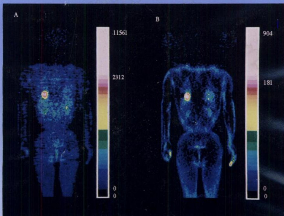
Attenuation-corrected (A) and uncorrected (B) ^{18}\text{F} -FDG images in a patient with adenocarcinoma of the lung. See pages 1219-1223.
