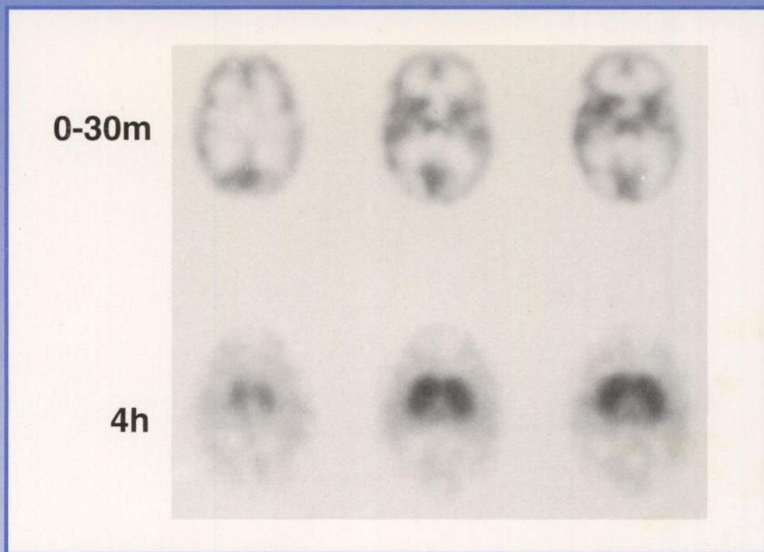
SPECT images of a human brain after intravenous injection of IBVM. See pages 405-410.
