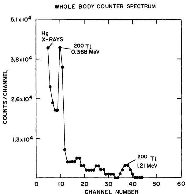
FIG. 1. Spectrum of thallium-200 as determined by Brookhaven National Laboratory whole-body counter. Mercury x-ray peak is not entirely shown because of cut-off by low-level discriminator.
