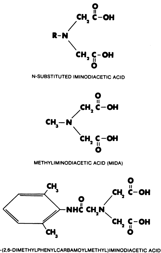
FIG. 1. Radiopharmaceuticals based on N-substituted iminodiacetic acids.
