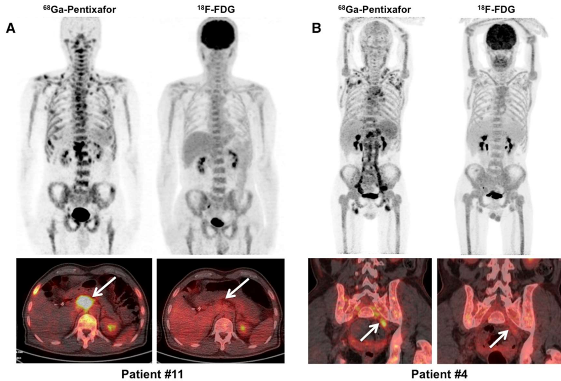
FIGURE 2. (A) Patient #11 had WM (IgM \lambda ), had an ISS-WM score of 2, and was classified as indeterminate risk. The ^{68}\text{Ga} -Pentixafor showed intense radioactivity in the bone marrow with multiple focal lesions and CXCR4-positive lymph nodes (arrow). The FDG activity (score 4) was homogeneously distributed in the bone marrow, and the lymph nodes were not FDG-avid (arrow). (B) Patient #4 had WM (IgM \kappa ) and Bing-Neel syndrome, had an ISS-WM score of 2, and was classified as indeterminate risk. Multiple CXCR4-positive lymph nodes were detected in the neck, axilla, hepatoduodenal, retroperitoneal, iliac, and inguinal regions, and most of these lymph nodes were missed with ^{18}\text{F} -FDG PET. The involved left iliac nerve root (arrow) was CXCR4-positive but not FDG-avid.
