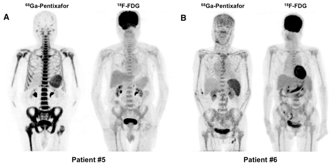
FIGURE 1. Examples of ^{68}\text{Ga} -Pentixafor and ^{18}\text{F} -FDG PET in patients with WM/LPL. (A) Patient #5 had relapsed WM (IgM \kappa ), had an ISS-WM score of 4, and was classified as high risk. The ^{68}\text{Ga} -Pentixafor showed intense radioactivity in the bone marrow that was much higher than ^{18}\text{F} -FDG (score 3). (B) Patient #6 had WM (IgM \kappa ) and secondary amyloidosis in the myocardium, had an ISS-WM score of 3, and was classified as high risk. The intensity of ^{68}\text{Ga} -Pentixafor and ^{18}\text{F} -FDG uptake in bone marrow was comparable, but the bone marrow involvement was more extensive with ^{68}\text{Ga} -Pentixafor than with ^{18}\text{F} -FDG. Additional bone marrow disease was detected in the craniofacial bones, ulna, radius, carpals and metacarpals with ^{68}\text{Ga} -Pentixafor. Note that the submandibular, retroperitoneal and inguinal lymph nodes were positive on ^{68}\text{Ga} -Pentixafor PET, but these lymph nodes were not FDG-avid.
