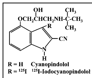
FIGURE 1. Schematic illustrations of cyanopindolol.
